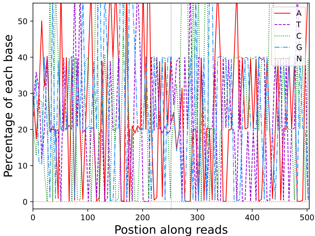
Base percentage along reads (R20106)
